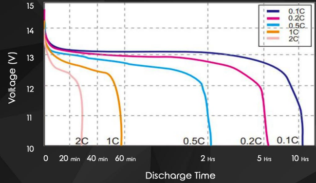
Different Rates Discharge Curve @ 25°C
