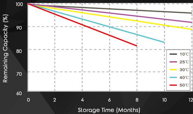
Different Temperatures Self Discharge Curve
