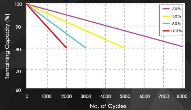
Different DOD Discharge Cycle Life Curve @ 1C
